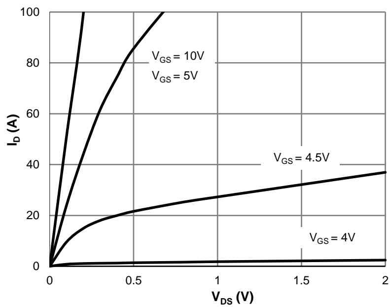
Figure 1: Saturation Characteristics
